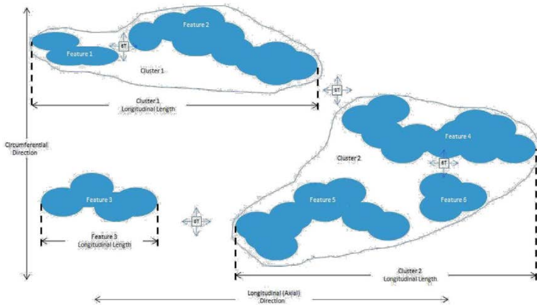
Enbridge Figure: Interacting Areas of Corrosion (2013)
